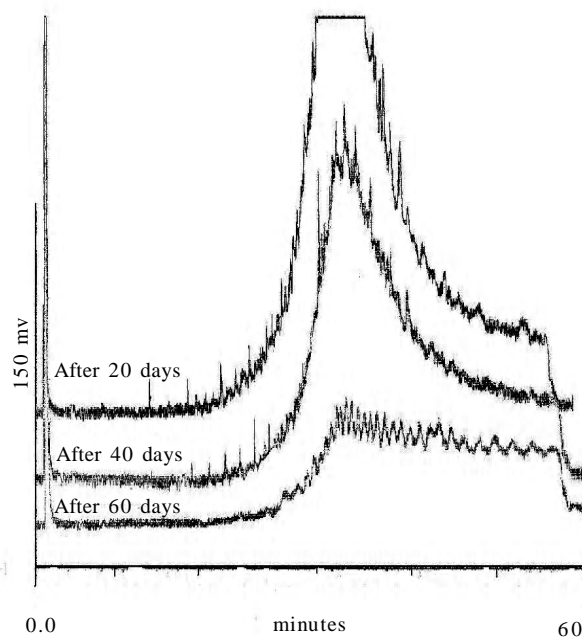
Fig. 10. GC chromatogram for samples extracted from contaminated soil treated by the mixed culture #1
