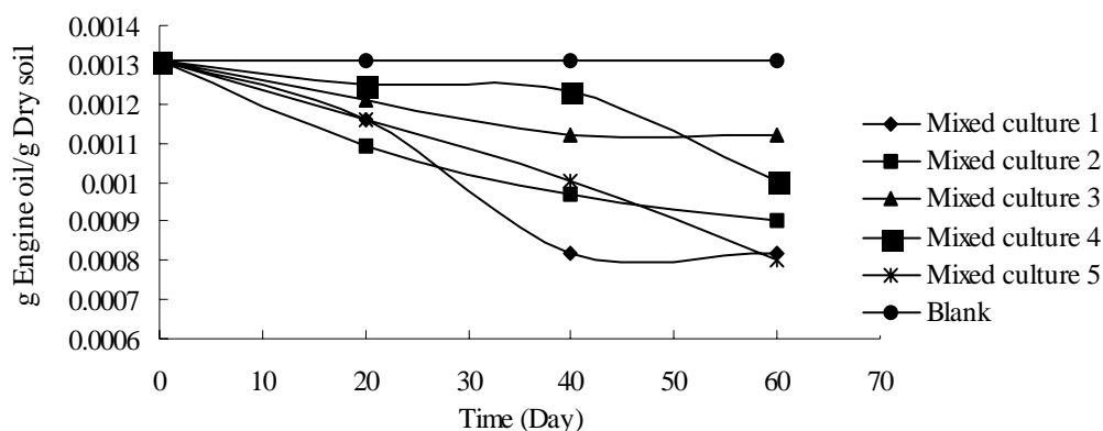
Fig. 8. Gravimetric experiments of aromatic engine oil compounds treated by the mixed consortia during 60 days
