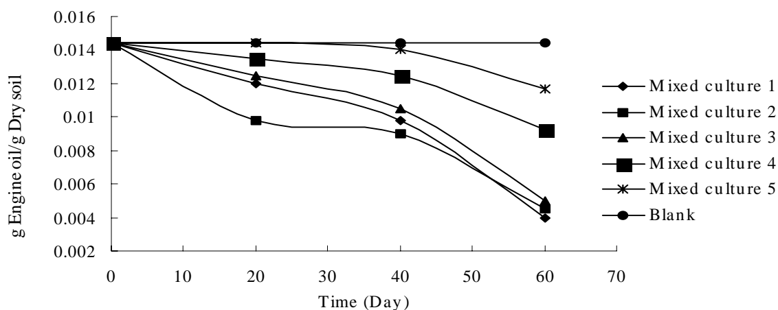
Fig. 4. Gravimetric experiments of engine oil treated by the mixed consortia during 60 days
