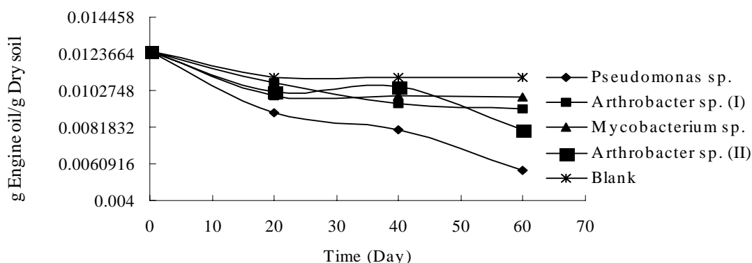
Fig. 5. Gravimetric experiments of aliphatic engine oil compounds treated by the isolated bacterial species during 60 days
