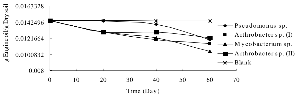
Fig. 3. Gravimetric experiments of engine oil treated by the isolated bacterial species during 60 days
