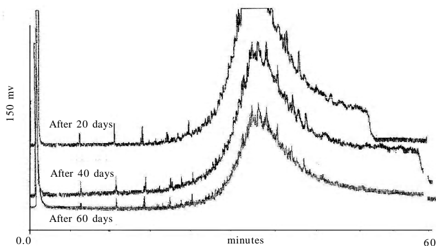
Fig. 11. GC chromatogram of sample extracted from contaminated soil treated by pure pseudomonas sp.
