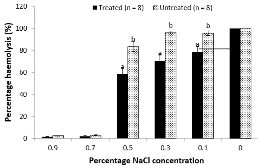
Fig. 3: Erythrocyte osmotic fragility of horses second week of supplementation with equithrive®. Values with different letters are significantly (P < 0.05) different.
