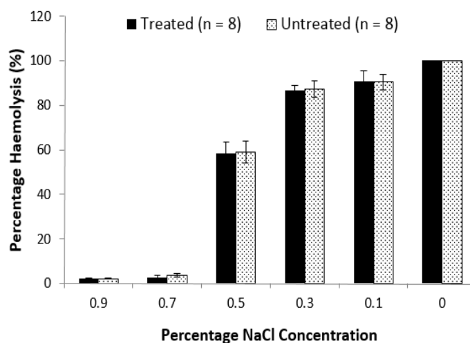
Fig. 1: Erythrocyte osmotic fragility of horses before supplementation
