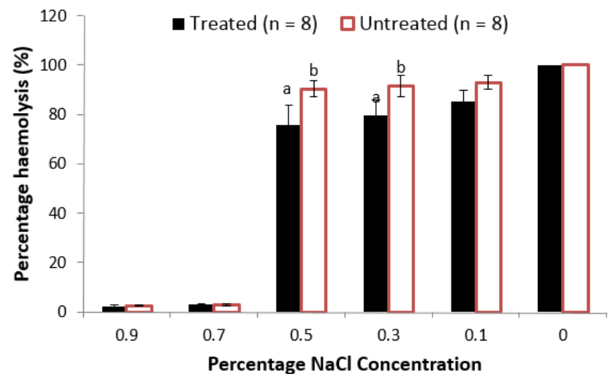
Fig. 4: Erythrocyte osmotic fragility of horses third week of supplementation with equithrive®. Values with different letters are significantly (P < 0.05) different.
