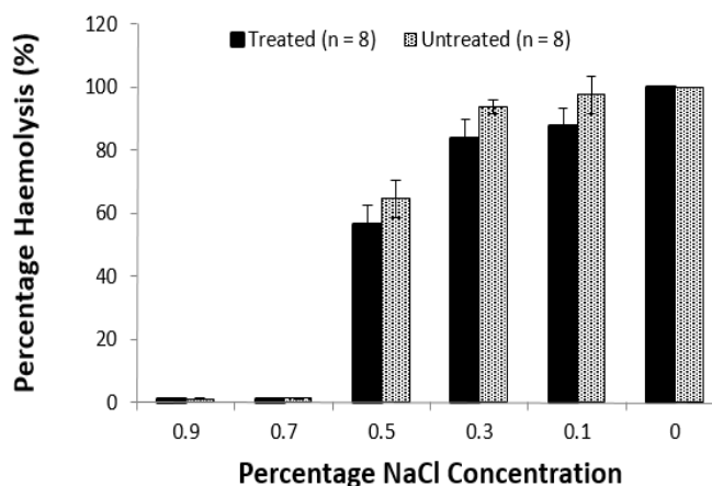
Fig. 2: Erythrocyte osmotic fragility of horses first week of supplementation with equithrive®. Values are not significantly ( P > 0.05 ) different
