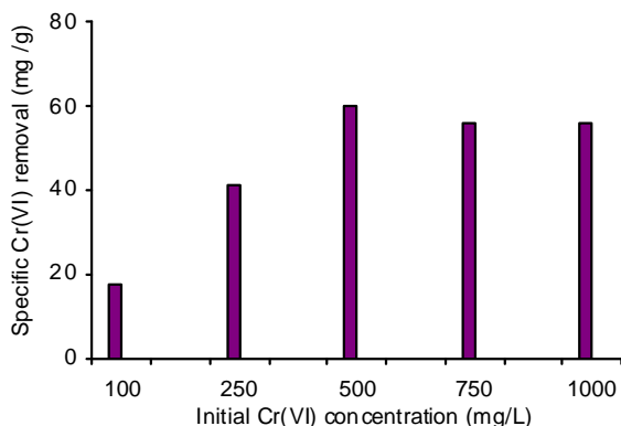
Fig. 2: Specific Cr (VI) removal at different initial Cr(VI) concentrations at pH=4
