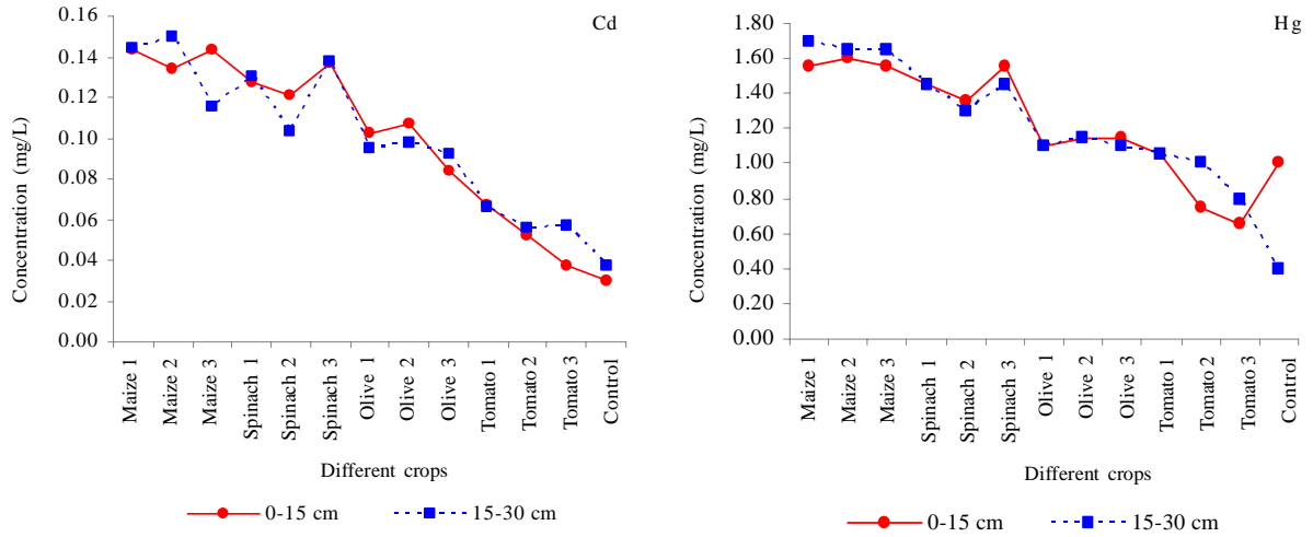
Fig. 1: Cd and Hg concentration in treated waste irrigated soils under different crops
