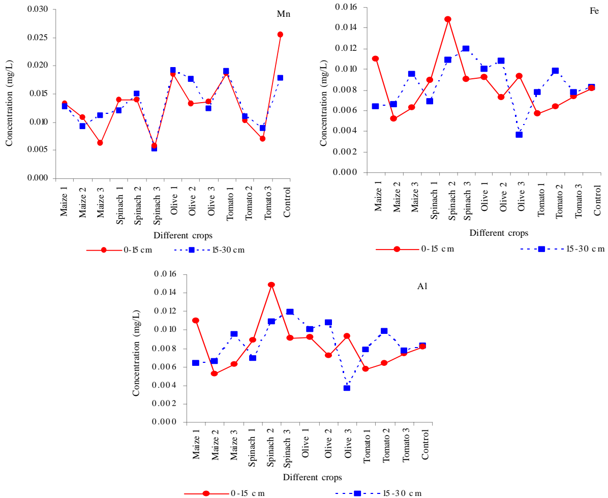
Fig. 4: Mn, Fe and Al concentration in treated waste irrigated soils under different crops
