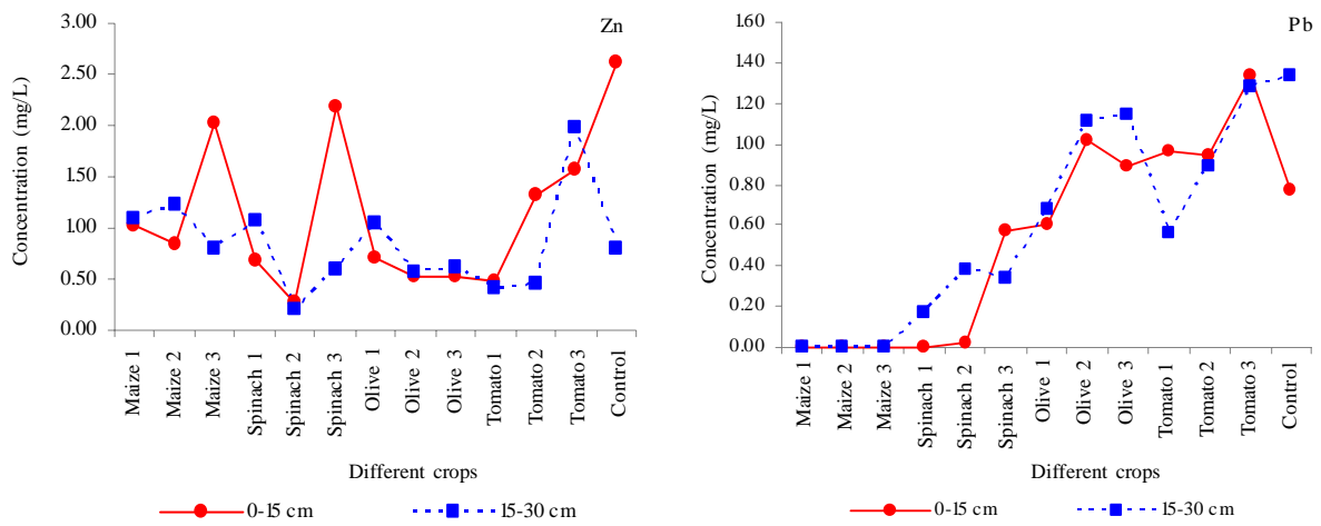
Fig. 3: Zn and Pb concentration in treated waste irrigated soils under different crops
