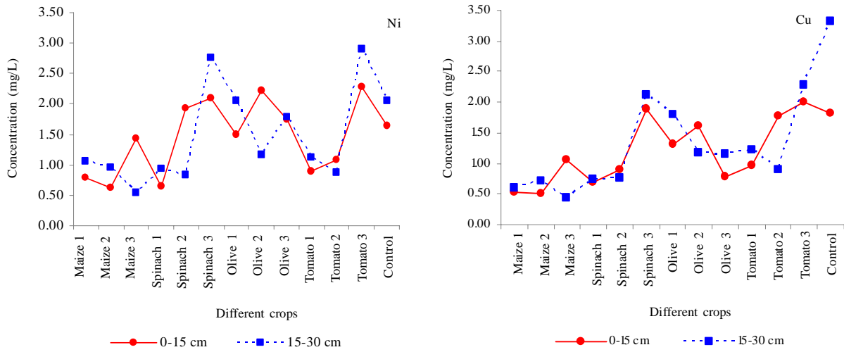
Fig. 2: Ni and Cu concentration in treated waste irrigated soils under different crops
