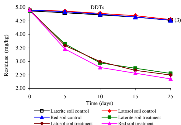
Fig. 2: Dynamic changes of residues of 4 components of DDT and DDTs in different types of soil
