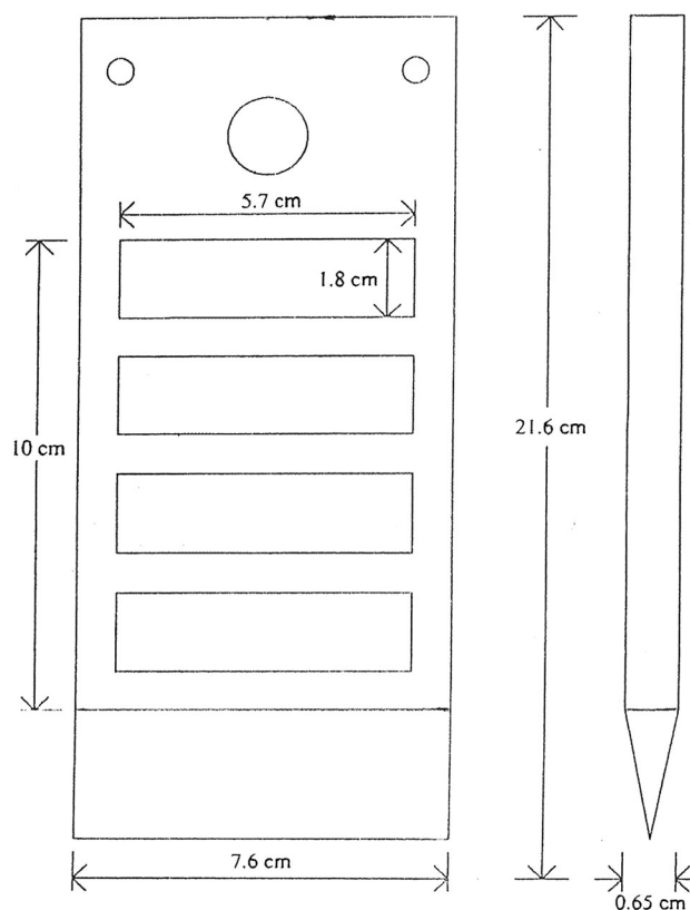
Fig. 1 Top and side view of dry deposition plate
