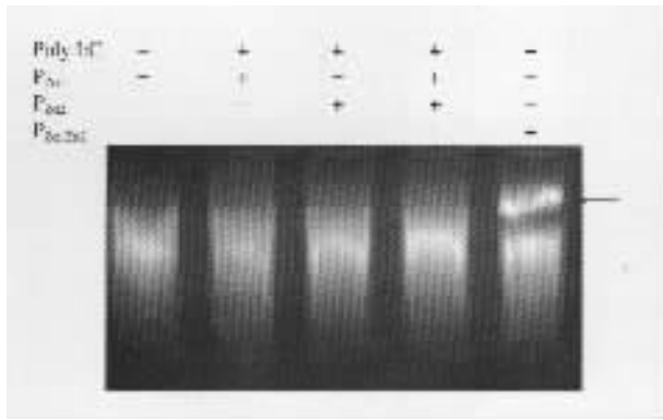
图 3 CaPKR-like Z\alpha 多肽与 Poly I:C 的凝胶阻滞分析 Fig. 3 Gel mobility shift assay for the binding of CaPKR-like Z\alpha fusion proteins to Poly I:C
