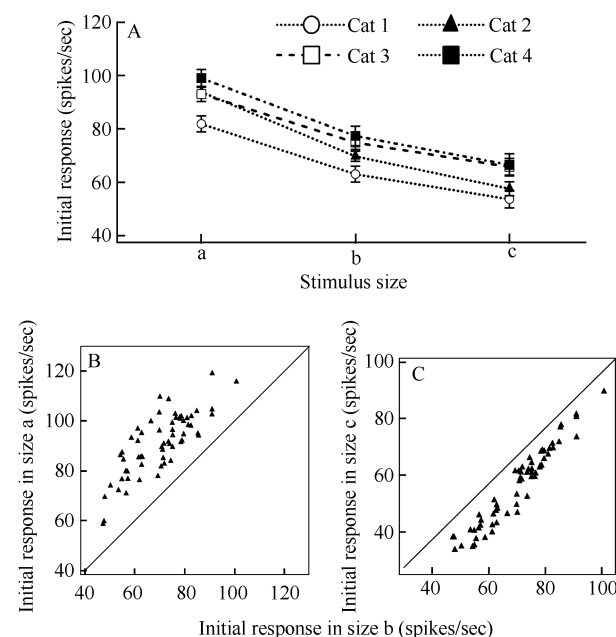
Figure 3 Average IR of neurons to prolonged visual stimuli with different sizes
