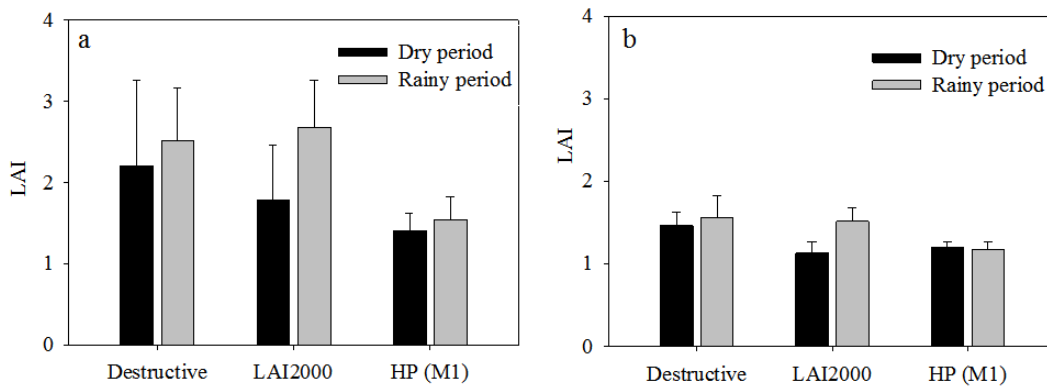
FIGURE 4: Averages of the measured (destructive) and estimated (LAI-2000 and Hemispherical Photos - HP) LAI data in the dry and rainy periods in the regions of Belo Oriente (a) and Antônio Dias (b).
