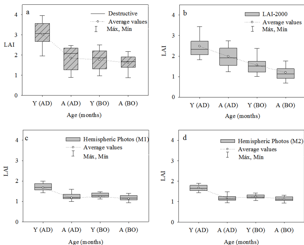
FIGURE 3: Average, maximum and minimum values, and the sampled quartiles for measurements of LAI by destructive (a) and indirect (b, c, d) methods in the stands found in the municipalities of Belo Oriente (BO) and Antônio Dias (AD) at young (Y) and adult (A) stands.
