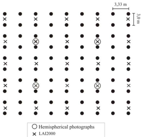
FIGURE 3: Sampling scheme performed by means of the LAI-2000 sensor and hemispherical cameras in the lines and between lines of the Eucalyptus stand.
